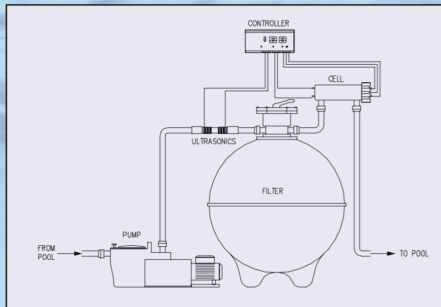
The EnviroSwim System
